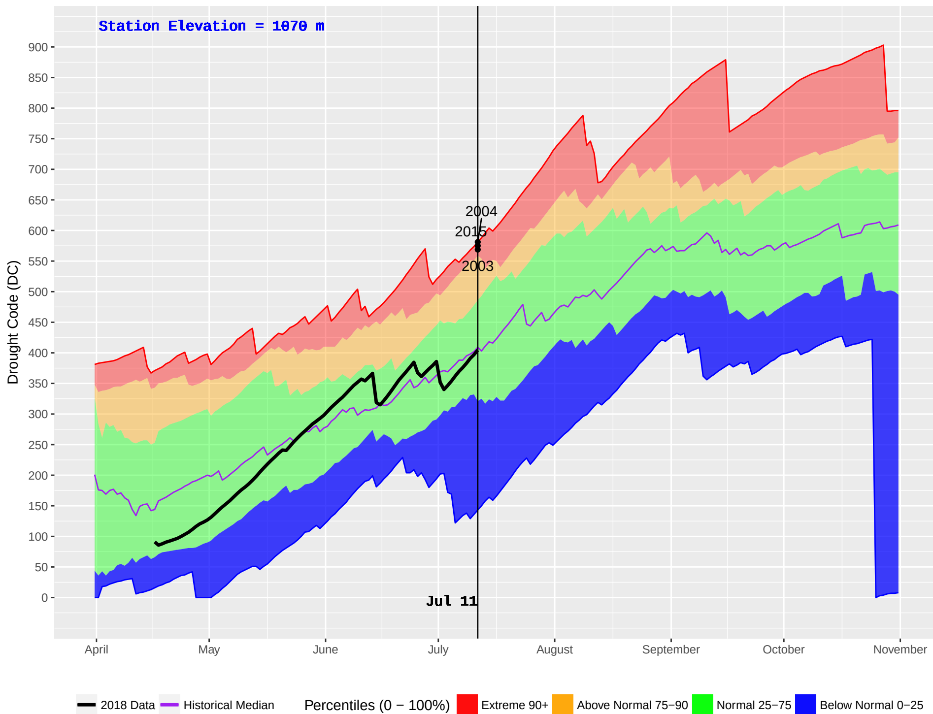
MEADOW LAKE (236) : Historical (1991–2016) and Current (2018) Noon Drought Code (DC)
