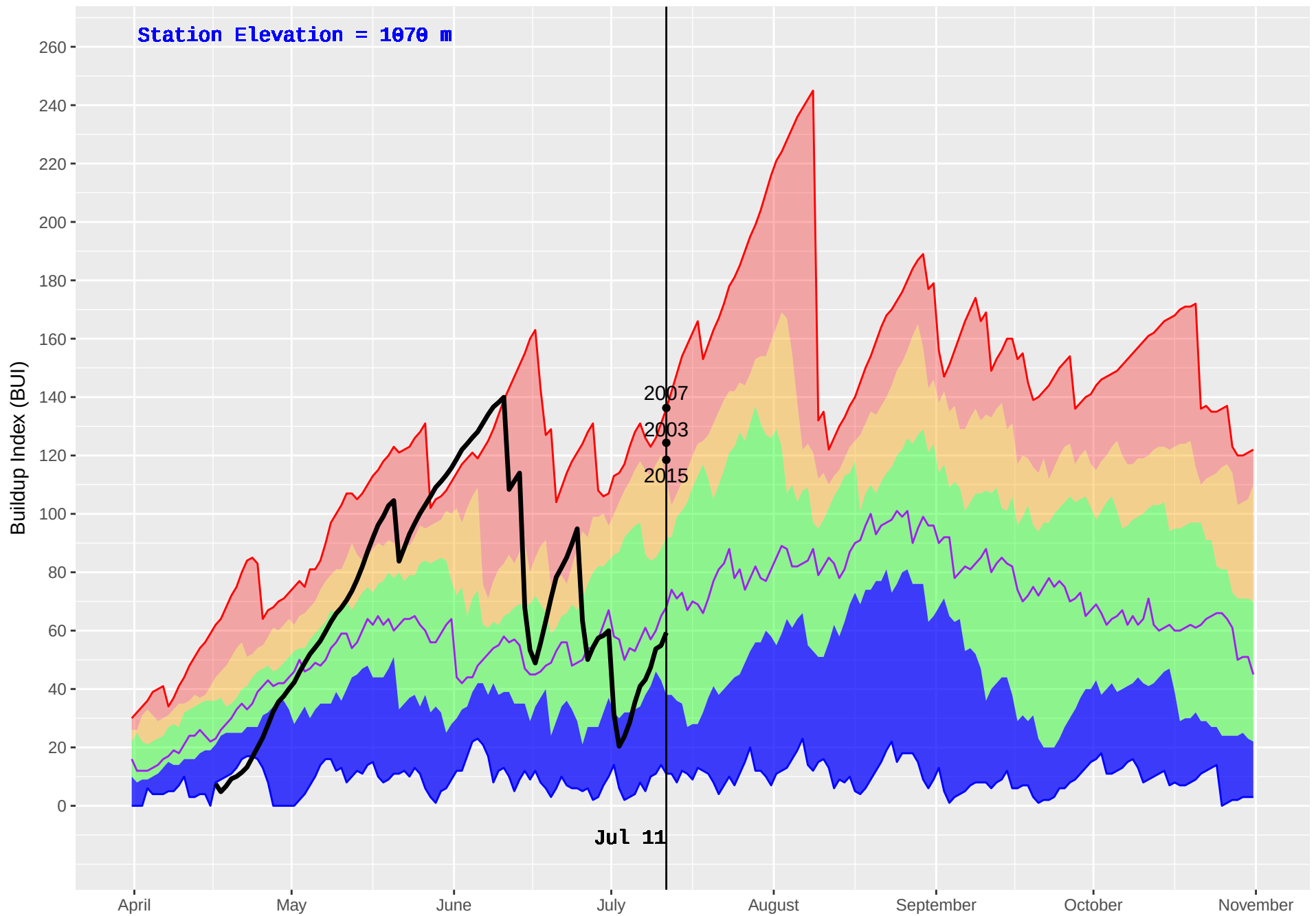
MEADOW LAKE (236) : Historical (1991–2016) and Current (2018) Noon Buildup Index (BUI)
