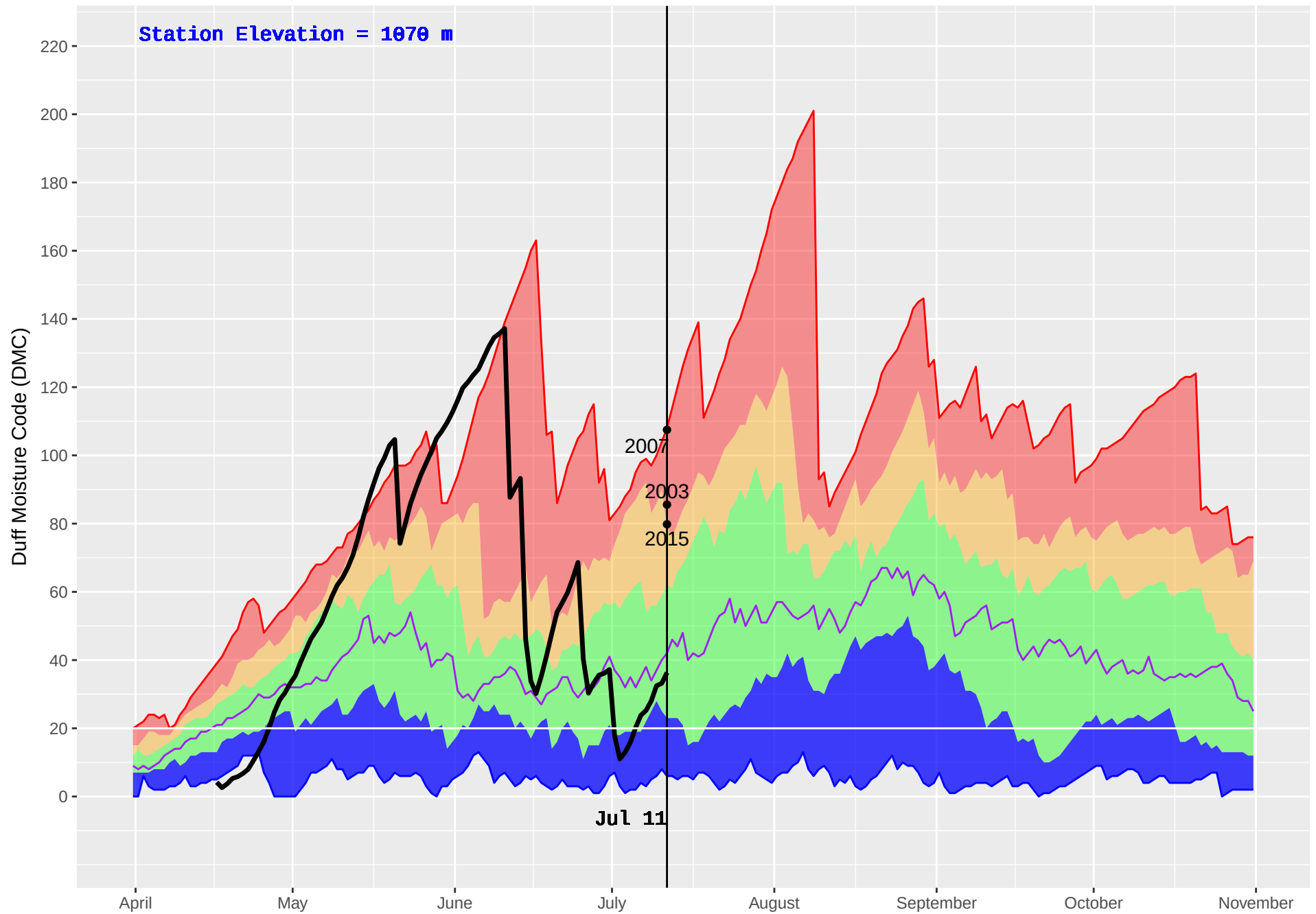
MEADOW LAKE (236) : Historical (1991–2016) and Current (2018) Noon Duff Moisture Code (DMC)
