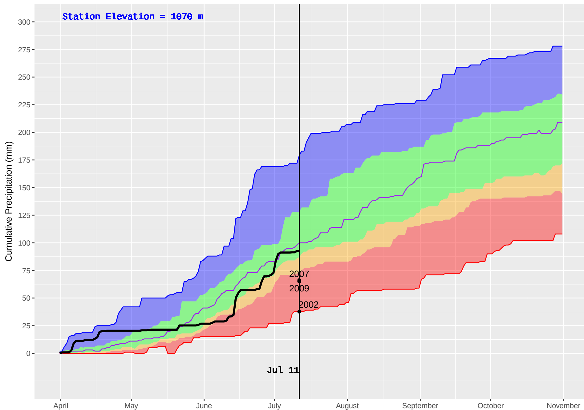
MEADOW LAKE (236) : Historical (1991–2016) and Current (2018) Noon Cumulative Precipitation
